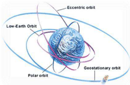
Fig 3: Different Orbits
